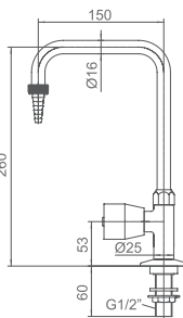
WJH0811 单联化验水咀 Single Assay Faucet
