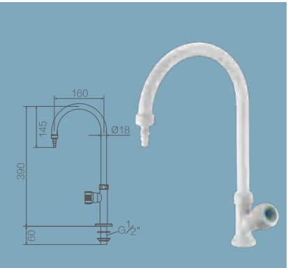
WJH0608C PP 单联化验水咀 PP Single Assay Faucet
