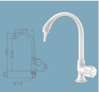
WJH0608B PP 单联化验水咀 PP Single Assay Faucet
