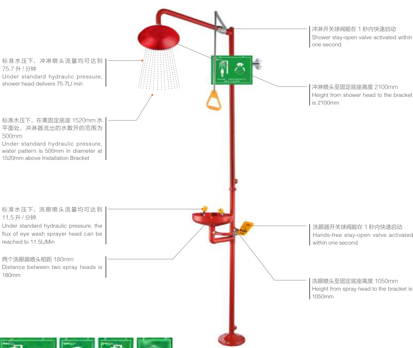
WJH0358A 不锈钢紧急冲淋洗眼器 Stainless Steel Emergency Shower & Eye Wash
