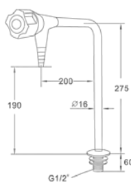
WJH0914 单联化验水咀 Single Assay Faucet
